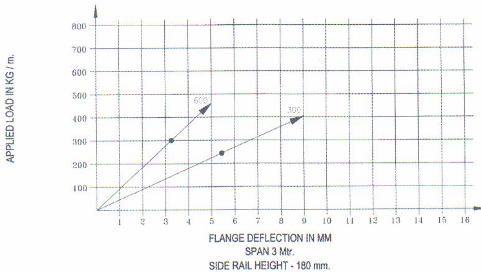
HEAVY DUTY CABLE LADDER
