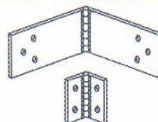
HORIZONTAL ADJUSTABLE CONNECTOR PART REFERENCE : HAC3
