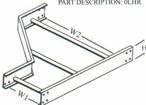
LEFT HAND REDUCER
